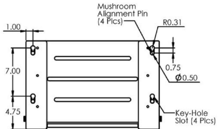
Rear View
