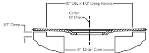
Cutaway Drain Detail
