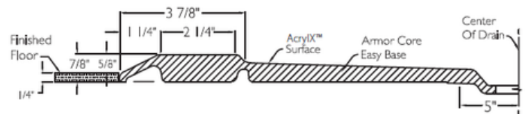
Right Drain Shown
