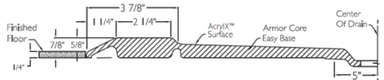
Right Drain Shown
