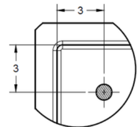
Standard Curtain Rod Location
