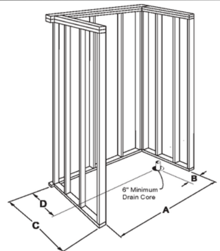
THRESHOLD VIEW
