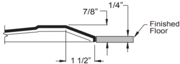
THRESHOLD VIEW
