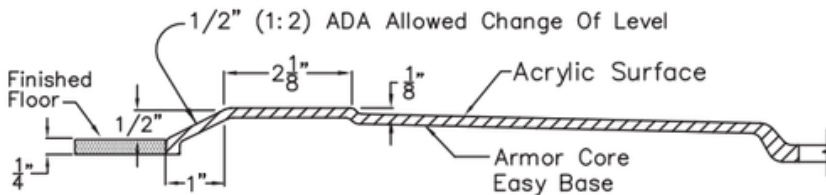
Detail of 3/4" Threshold
