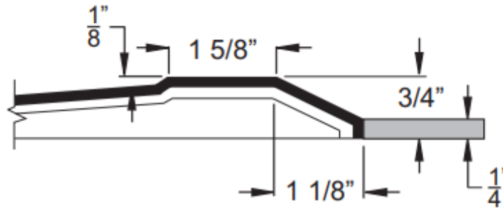
THRESHOLD VIEW
