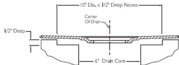
COMES WITH NO CAULK DRAIN and Square Strainer Plate Cutaway Drain Detail
